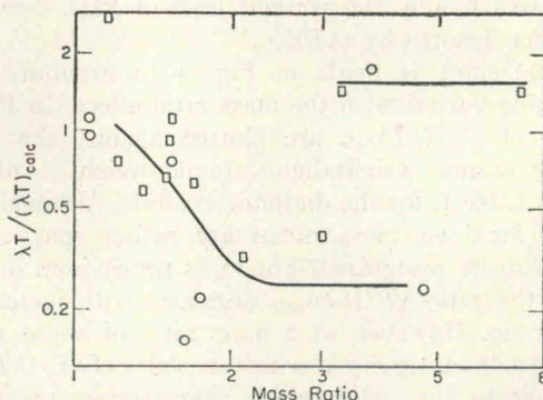
FIG. 4. The deviations of the points from the lines of Figs. 2 and 3, \lambda T / (\lambda T)_{\text{calc}} , plotted against the ratio (heavy atomic weight/light atomic weight) for the diatomic crystals.
